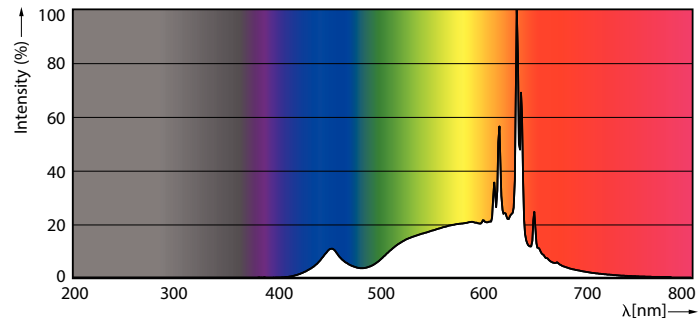
LEDspots Corepro SLR 3W PAR16 GU10 827 36D-POC
